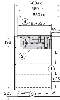
KMDA7272FL, KMDA7473FL – Side view lying on top+X, Plug&Play – Installation drawing
